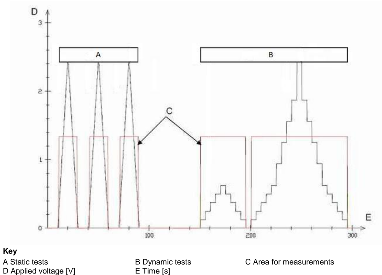
Figure 7: Electrical cycle
