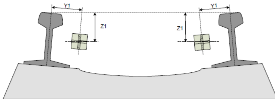
Figure 12: Position of the measurement antenna (internal between the rails)
